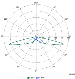
Polar Normal (separate) - BDP768I - 912300024527
