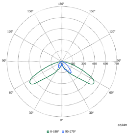
Polar Normal (separate) - BDP768I - 912300060155
