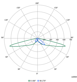
Polar Normal (separate) - BDP768I - 912300024528
