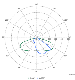
Polar Normal (separate) - BGP280I - 910925869157
