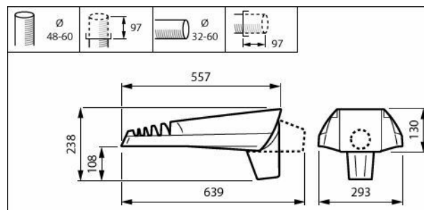
BGP702 LED40-4S/740 DM10 PGR SRT SRB 60
