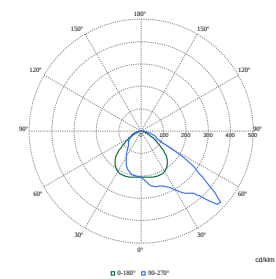
Polar Normal (separate) - BVP125I - 912300060603
