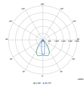
Polar Normal (separate) - BVP125I - 912300057767
