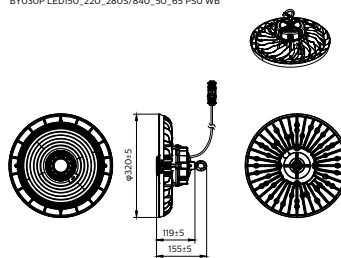
BY030P LED150_220_2805/840_50_65 PSU WB
