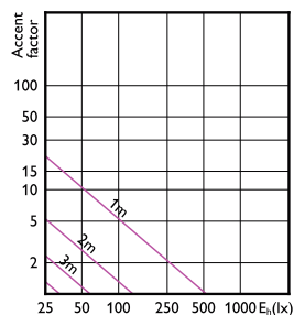
Accent Diagram - CorePro LED spot ND 2.9-20W MR16 827 36D
