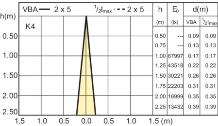
Beam diagram - MASTERC CDM-R 70W/830 E27 PAR30L 10D 1CT
