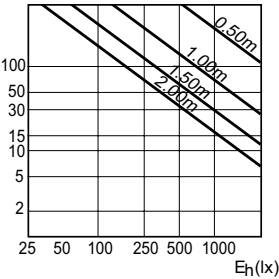
Accent Diagram - MASTERC CDM-R 70W/830 E27 PAR30L 10D 1CT
