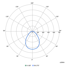
Polar Normal (separate) - DN145BI - 910500465903
