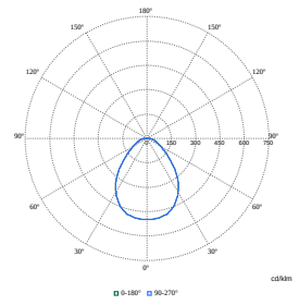
Polar Normal (separate) - DN145BI - 910505101196
