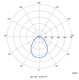
Polar Normal (separate) - DN145BI - 910505101198
