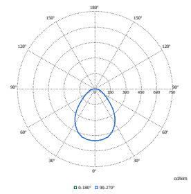
Polar Normal (separate) - null - 911401816285
