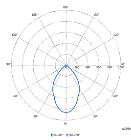
Polar Normal (separate) - DN460BN - 912500100535
