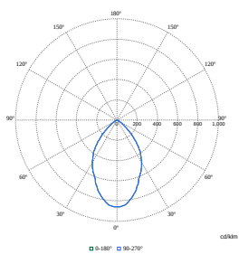
Polar Normal (separate) - DN460BN - 910505102098
