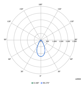
Polar Normal (separate) - DN460BN - 912500100519
