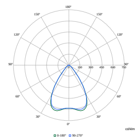
Polar Normal (separate) - DN572BI - 910505100942
