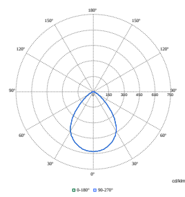
Polar Normal (separate) - DN570BI - 910505100869
