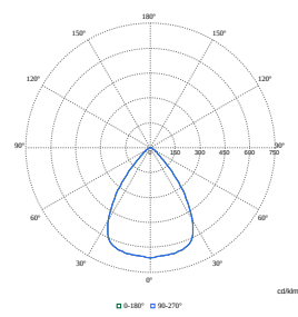
Polar Normal (separate) - DN570BI - 910505100840
