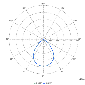
Polar Normal (separate) - DN570BI - 910505100845
