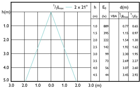
Beam diagram - MAS LED spot VLE D 7-80W GU10 940 36D
