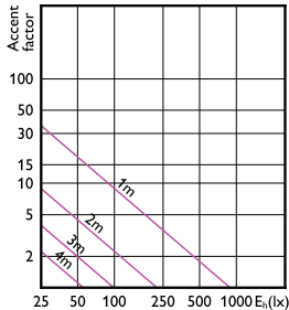
Accent Diagram - MAS LED spot VLE D 7-80W GU10 940 36D
