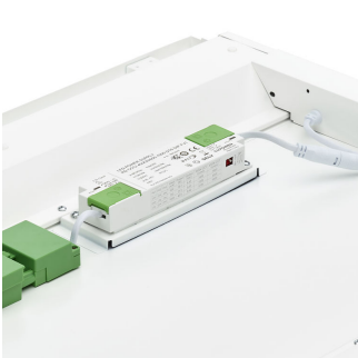
CoreLine recessed G4 PSD W60L60 back side detail dipswitches
