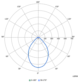
Polar Normal (separate) - RC450BI - 910505103947
