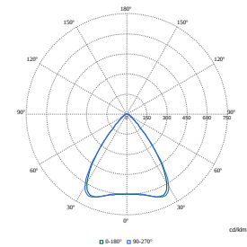
Polar Normal (separate) - RC450BI - 910505103974
