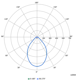
Polar Normal (separate) - RC450BI - 910505103941
