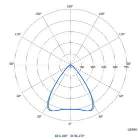
Polar Normal (separate) - RC450BI - 910505103972
