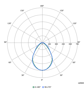
Polar Normal (separate) - RC450BI - 910505103951
