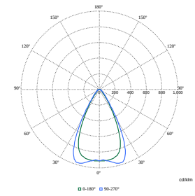
Polar Normal (separate) - RC450BI - 910505105906
