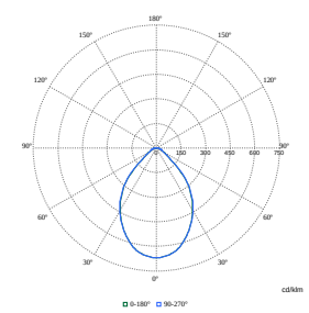
Polar Normal (separate) - RC450BI - 910505103947
