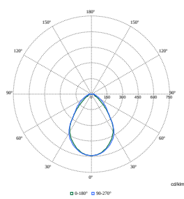
Polar Normal (separate) - RC450BI - 910505103953
