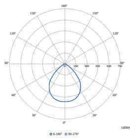
Polar Normal (separate) - RC460BN - 910505100422
