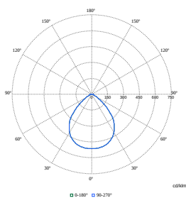
Polar Normal (separate) - RC460BN - 910505103639
