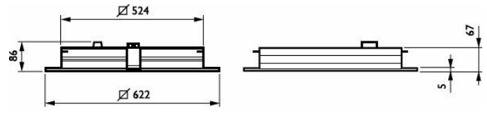
RC463B 34S/840 SEIA W62L62 VPC U4 UE
