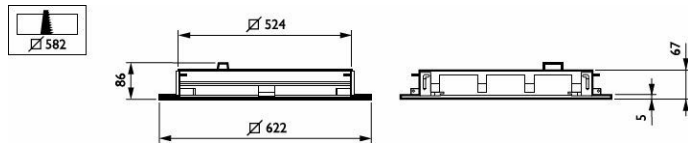
RC463B 34S/940 DEIA W62L62 CPC
