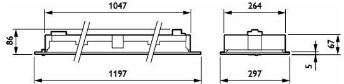
RC461B 80S/TW9 SEIA W30L120 VPC CWL U4
