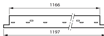
Recessed VPC_W8L120_sensor/IP
