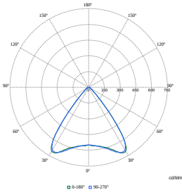
Polar Normal (separate) - RC530BI - 910505103150
