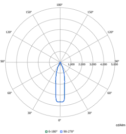
Polar Normal (separate) - RS320BI - 910505102991
