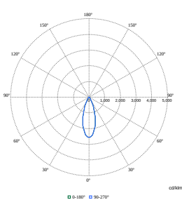
Polar Normal (separate) - RS353BI - 910505102759
