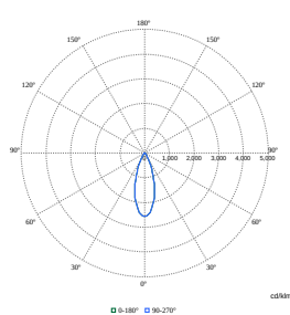
Polar Normal (separate) - RS353BI - 910505102758
