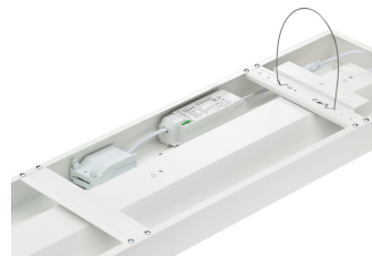
CoreLine surface mounted G4 PSU back side
