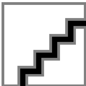
Polar Normal (separate) - null - 912401483455
