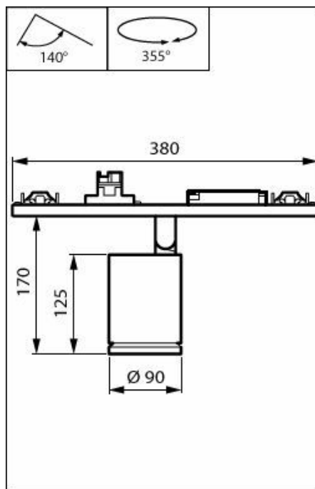
ST770X 17S/830 DIA MB FG WH
