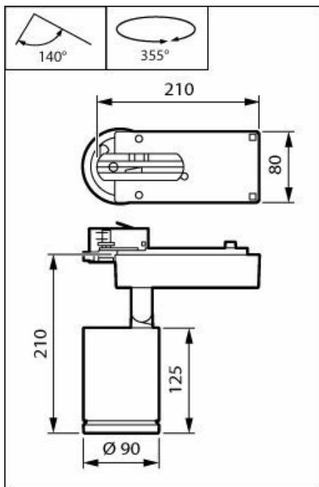
ST770T 39S/PC930 PSU MB FG BK
