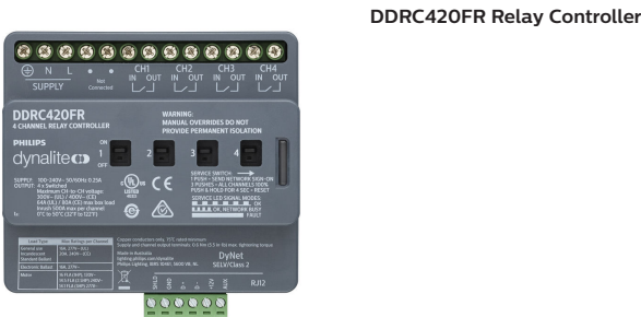
DDR420FR Relay Controller
