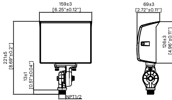
20W Knuckle SlimFlood 10-15-20W/3CCT/UN3/KN
