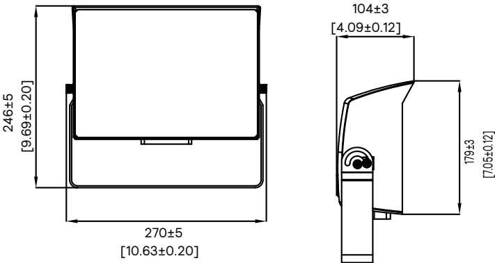
80W Yoke SlimFlood 60-70-80W/3CCT/UN3/YK/PCB
