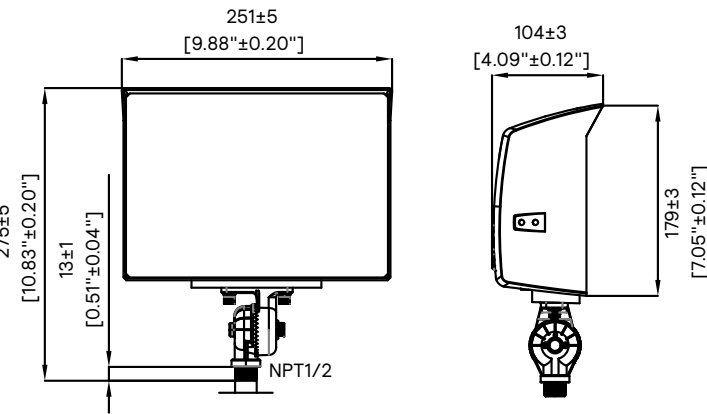
80W Knuckle SlimFlood 60-70-80W/3CCT/UN3/KN/PCB
