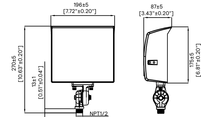
60W Knuckle SlimFlood 34-45-60W/3CCT/UN3/KN/PCB
