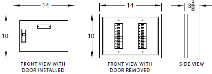
Flanged Trim Panel - up to 16 Circuits
