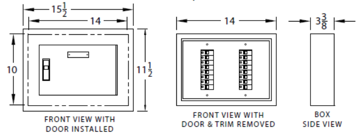
Flush Trim Panel - up to 16 Circuits
