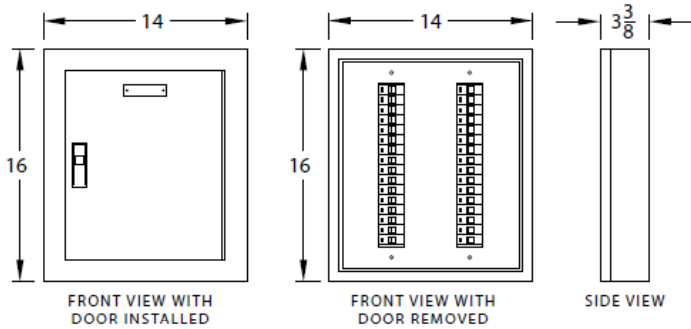
Flanged Trim Panel - up to 32 Circuits
