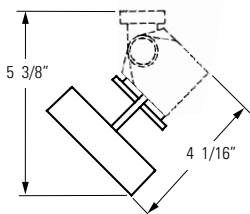
Ring PAR20 with Par-Tech® Incandescent/halogen Fixture 8201
