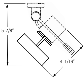
Ring PAR20 with Par-Tech® Incandescent/halogen Fixture 8202
