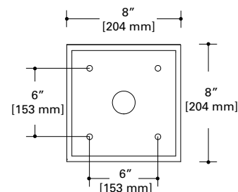
Mounting Plate
