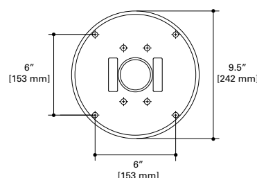
Mounting Plate
