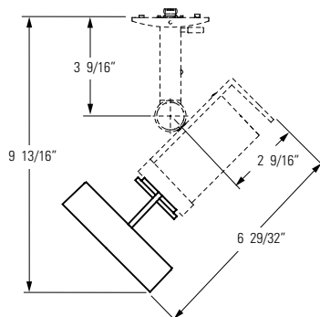
Ring PAR20 with Metalics™ Incandescent/Halogen Fixtures 8701 & 28701 (ProSpec)
