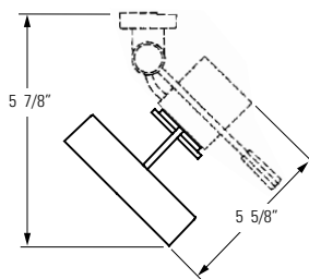
Ring PAR30 with Par-Tech® Incandescent/halogen Fixture 8202
