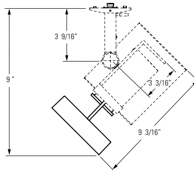
Ring PAR20 with Metalics™ Electronic Metal Halide Fixtures 8704E, 8705E, & 28705E (prospec)
