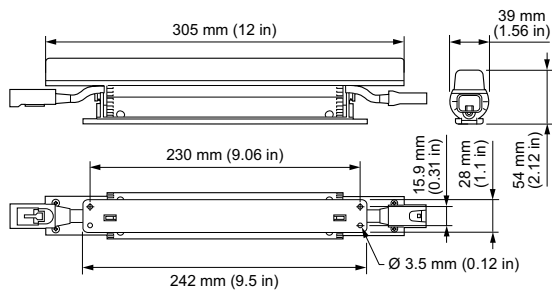
LS515X LED5/3500 100-277V MB WH
