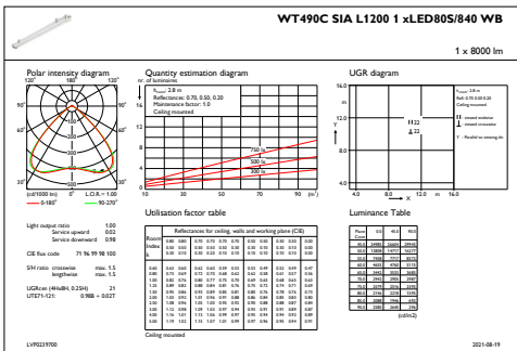
IFGU1_WT490CSIAL12001xLED80S840WB
