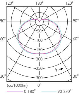
Light Distribution Diagram - Corepro LED T25 ND 3.2-25W E14 827
