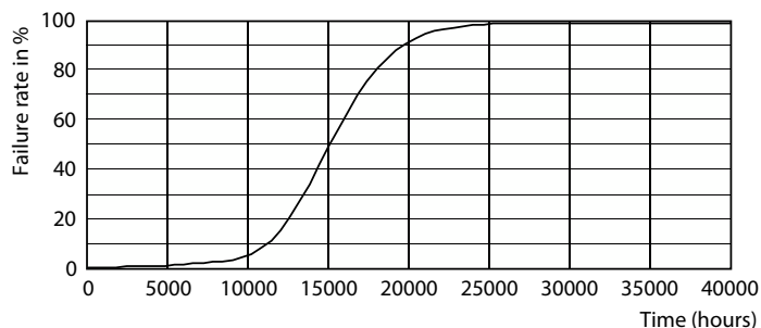
Life Expectancy Diagram - MAS LED D2D ND 7.5-60W A60 E27 827
