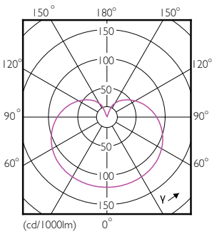
Light Distribution Diagram - MAS LED D2D ND 7.5-60W A60 E27 827
