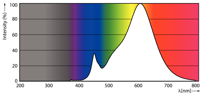
Spectral Power Distribution Colour - MAS LED D2D ND 7.5-60W A60 E27
