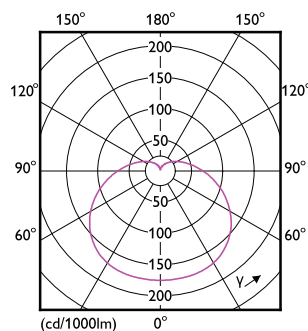
Light Distribution Diagram - ESS LEDBulb 9W E27 6500K 230V 1CT/12 CN
