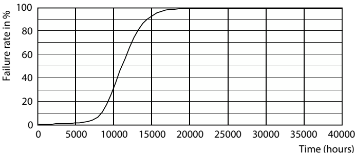
Life Expectancy Diagram - ESS LEDBulb 9W E27 6500K 230V 1CT/12 CN
