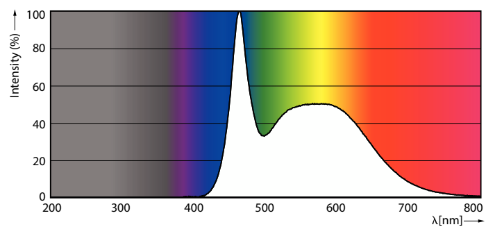
Spectral Power Distribution Colour - ESS LEDBulb 9W E27 6500K 230V 1CT/12 CN
