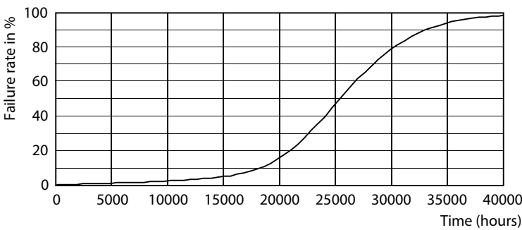
Life Expectancy Diagram - DL252 G2 R SQ LED 1300 65K 18W 8" WV 1pk
