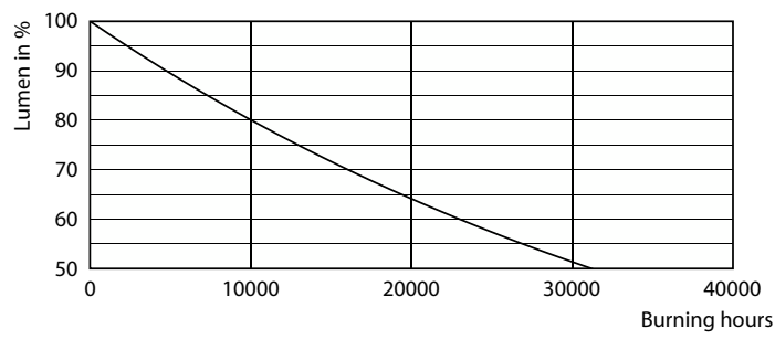
Lumen Maintenance Diagram - TForce Core HB 30W E27 865 GN3
