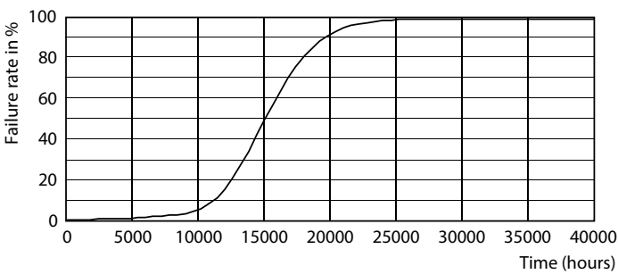
Life Expectancy Diagram - TForce Core HB 30W E27 865 GN3
