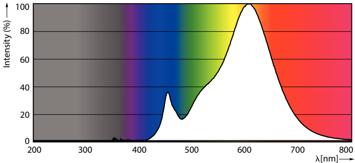
Spectral Power Distribution Colour - LEDGlobe 10-75W G120 E27 WW 230V_AU
