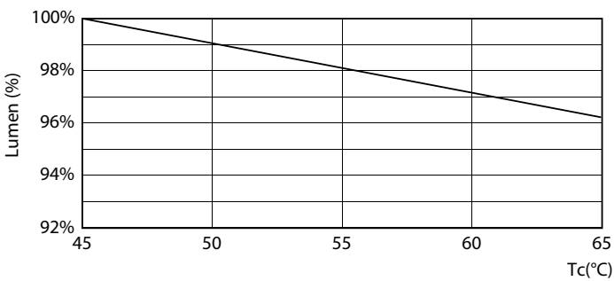
Lumen Maintenance Diagram - 16.9T8/MAS/48-850/MF25/P 10/1
