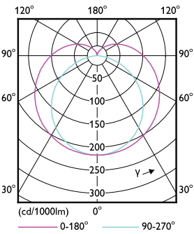
Light Distribution Diagram - 16.9T8/MAS/48-850/MF25/P 10/1
