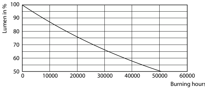
Lumen Maintenance Diagram - MAS LEDcandle DT 2.8-25W E14 B38 CL
