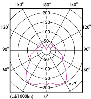
Light Distribution Diagram - MAS LEDcandle DT 2.8-25W E14 B38 CL
