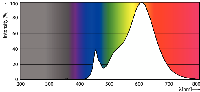
Spectral Power Distribution Colour - MAS LEDcandle DT 2.8-25W E14 B38 CL
