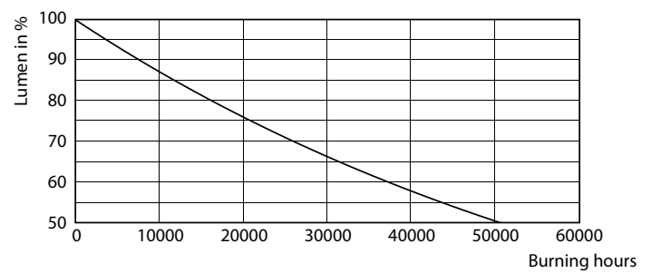
Lumen Maintenance Diagram - MAS LEDlustre DT 8-60W P50 E14 827 CL
