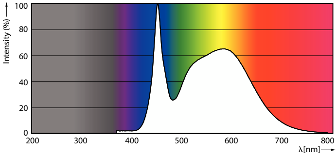
Spectral Power Distribution Colour - 165HB/LED/850/D WB UDL BB G2 4/1
