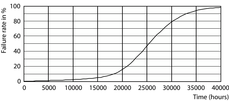
Life Expectancy Diagram - DL252 G2 SF SQ LED 900 30K 12W 6" WV
