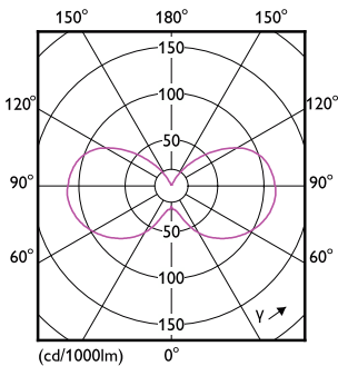
Light Distribution Diagram - 5BA11/PER/UD/CL/G/E26/WGD 6/3PF T20
