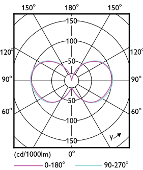
Light Distribution Diagram - 63CC/LED/850/LS EX39 G3 BB 3/1
