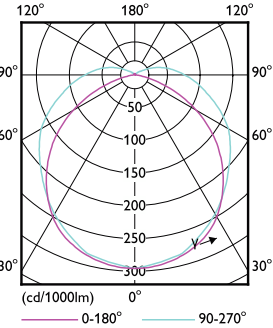
Light Distribution Diagram - 40WP/LED/840/LS EX39 G3 BB 3/1
